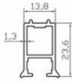
K4405 SABİT DİKME (0.260 Kg/m)
