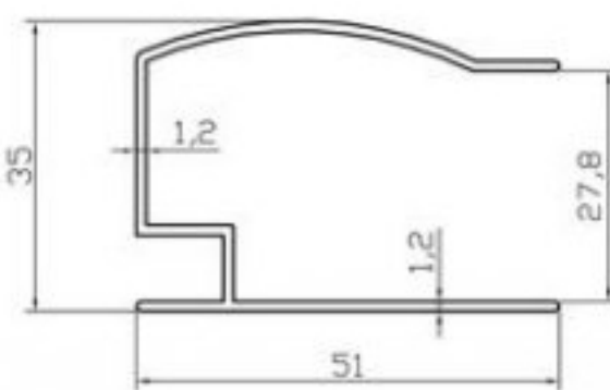
K4426 CAM DİKME PROFİLİ 0.470 Kg/m
