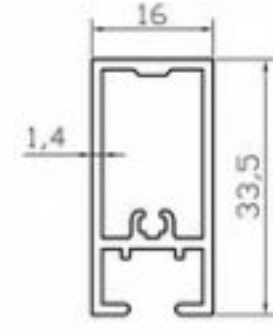
K4406 ASKILIK PROFİLİ (0.430 Kg/m)
