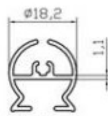
K4424 ARA FİTİLLİ DİKME (0.245 Kg/m)
