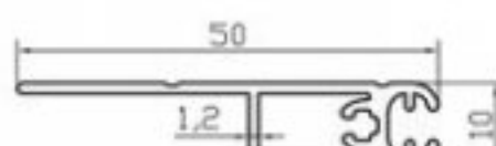
K4423 ASKILIK PROFİLİ (0.355 Kg/m)
