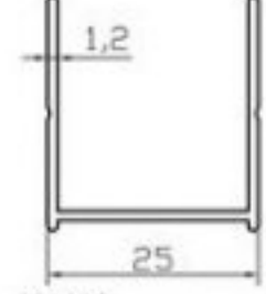
K4412 DUVAR DİKME PROFİLİ (0.240 Kg/m)
