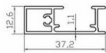
K4407 İÇ RAY PROFİLİ (0.320 Kg/m)
