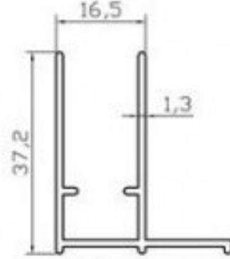
K4409 DUVAR DİKME (0.390 Kg/m)
