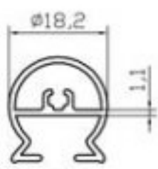
K4400 FİTİLSİZ DİKME (0.215 Kg/m)
