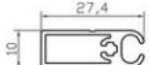
K4418 SABİT DİKME (0.290 Kg/m)
