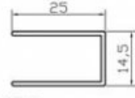
K4415 DUVAR DİKME PROFİLİ (0.200 Kg/m)
