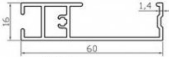
K4408 ASKILIK PROFİLİ (0.540 Kg/m)
